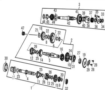
FIG. 10 TRANSMISION
