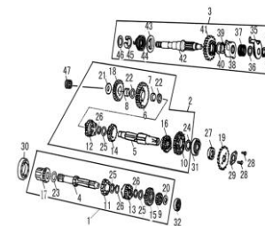
FIG. 9 TRANSMISION
